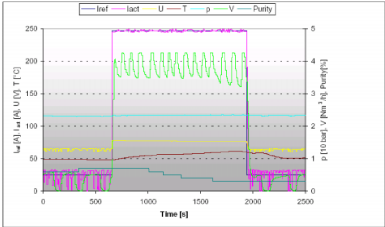
Figure 5: Load change of 90%
