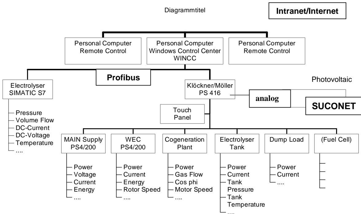
Figure 12: Structure of the data collection system
