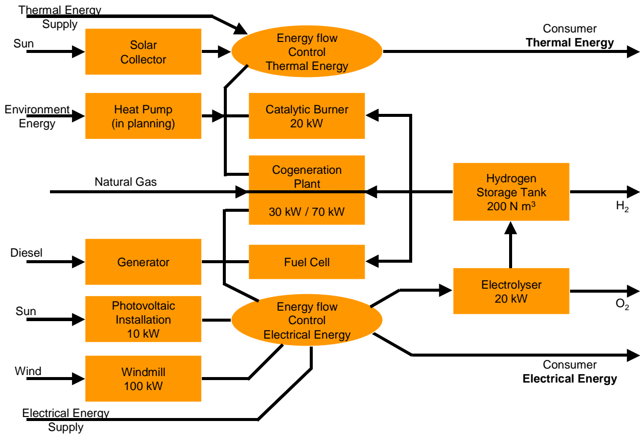
Figure 1: Components and their integration in the Multi-component Laboratory
