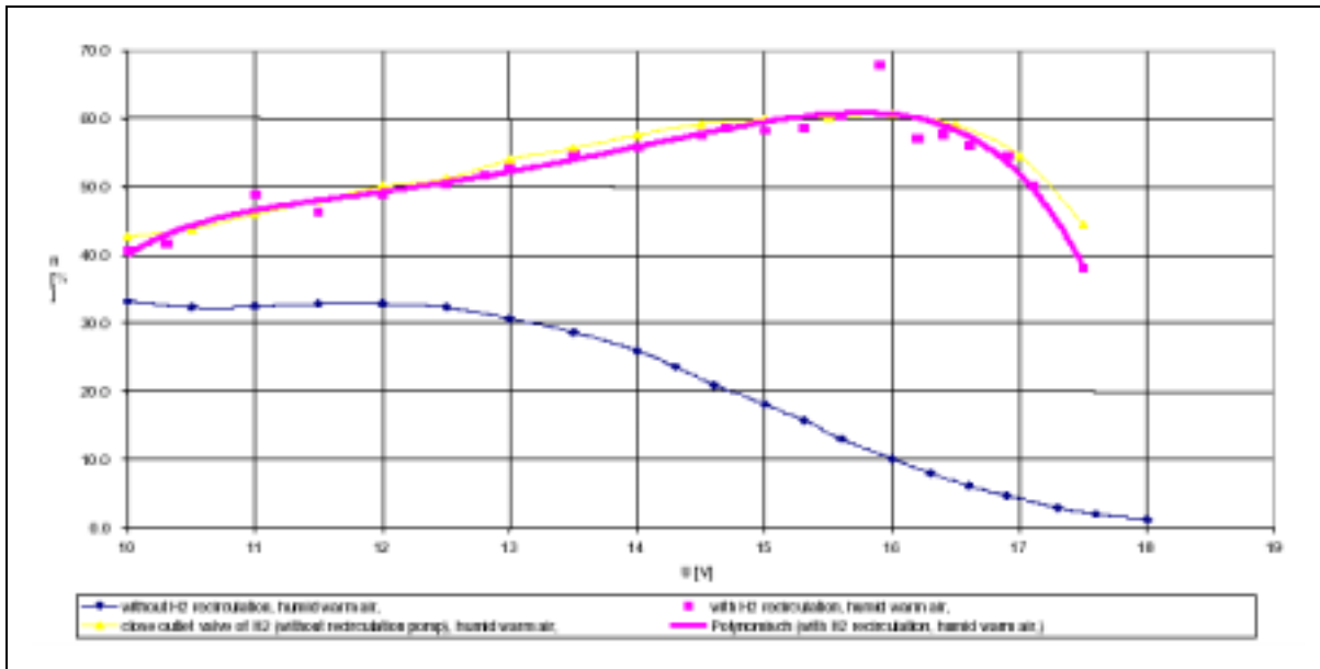
Figure 10: Fuel cell efficiency depending on the voltage
