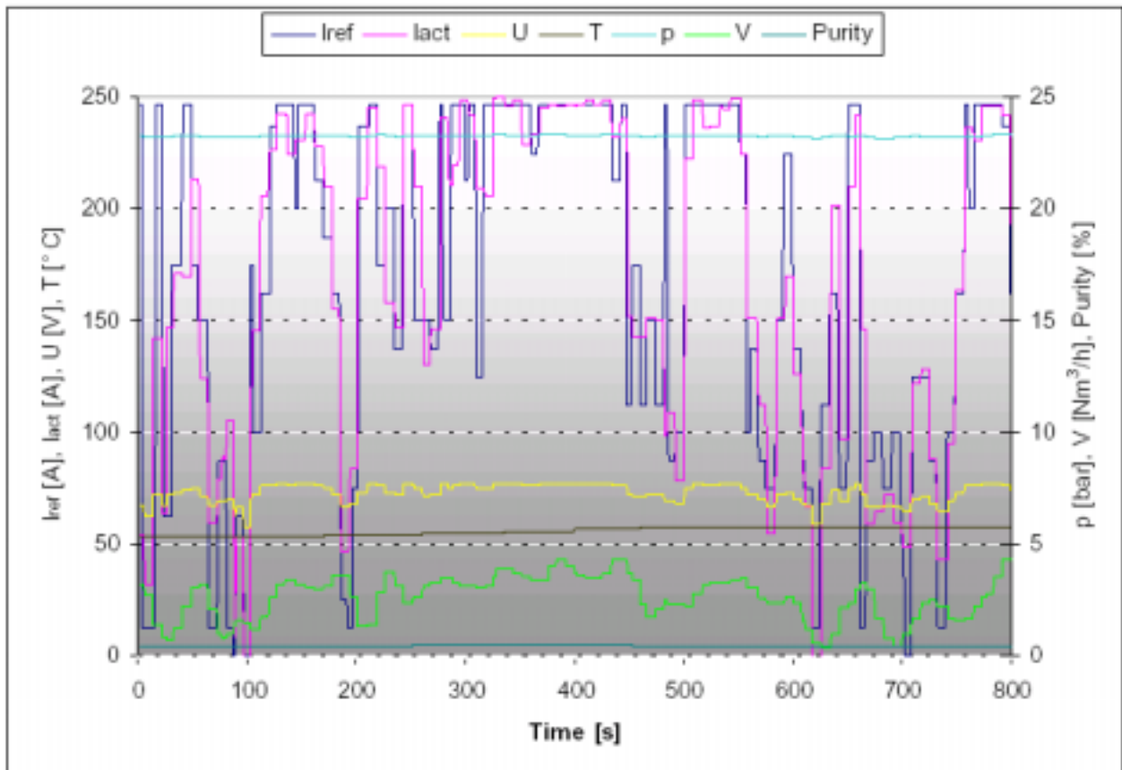
Figure 6: Windmill controlled electrolyser
