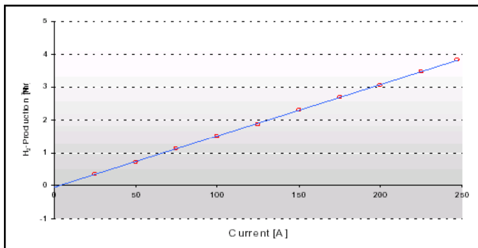
Figure 4: Hydrogen production
