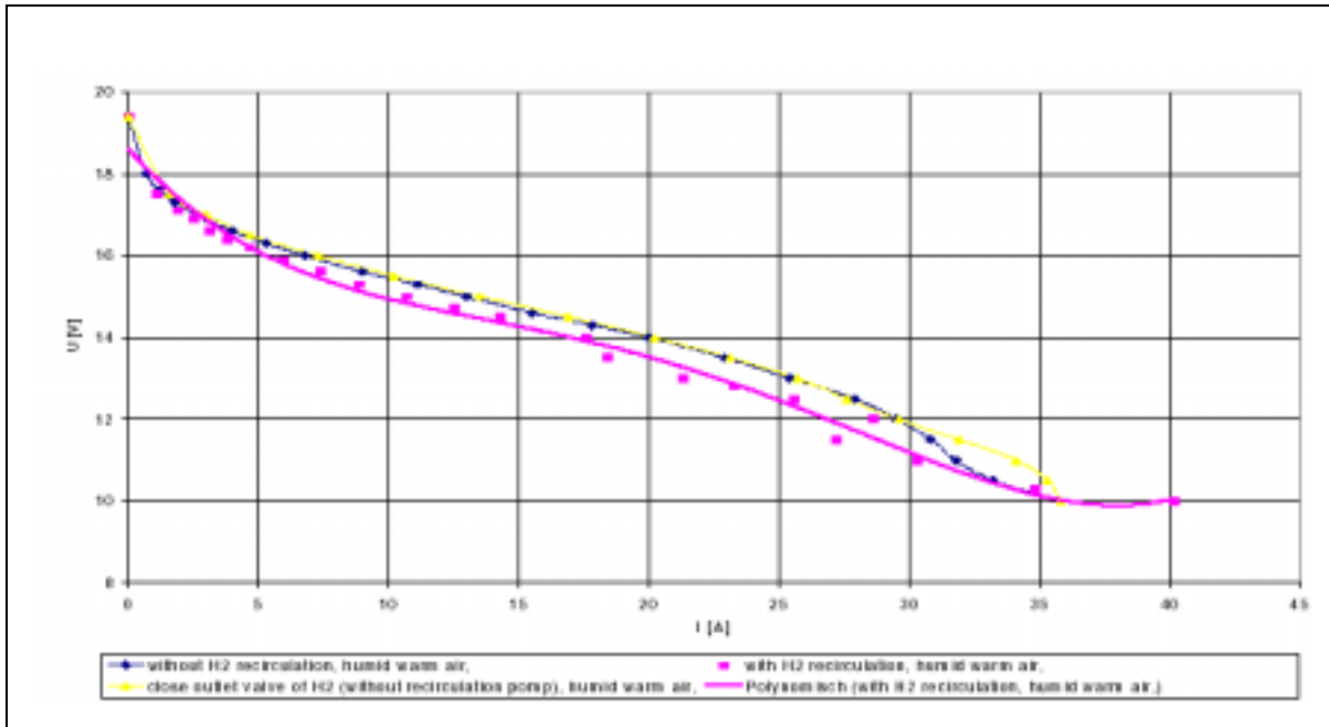
Figure 8: Voltage/current diagram of the PEM Fuel Cell
