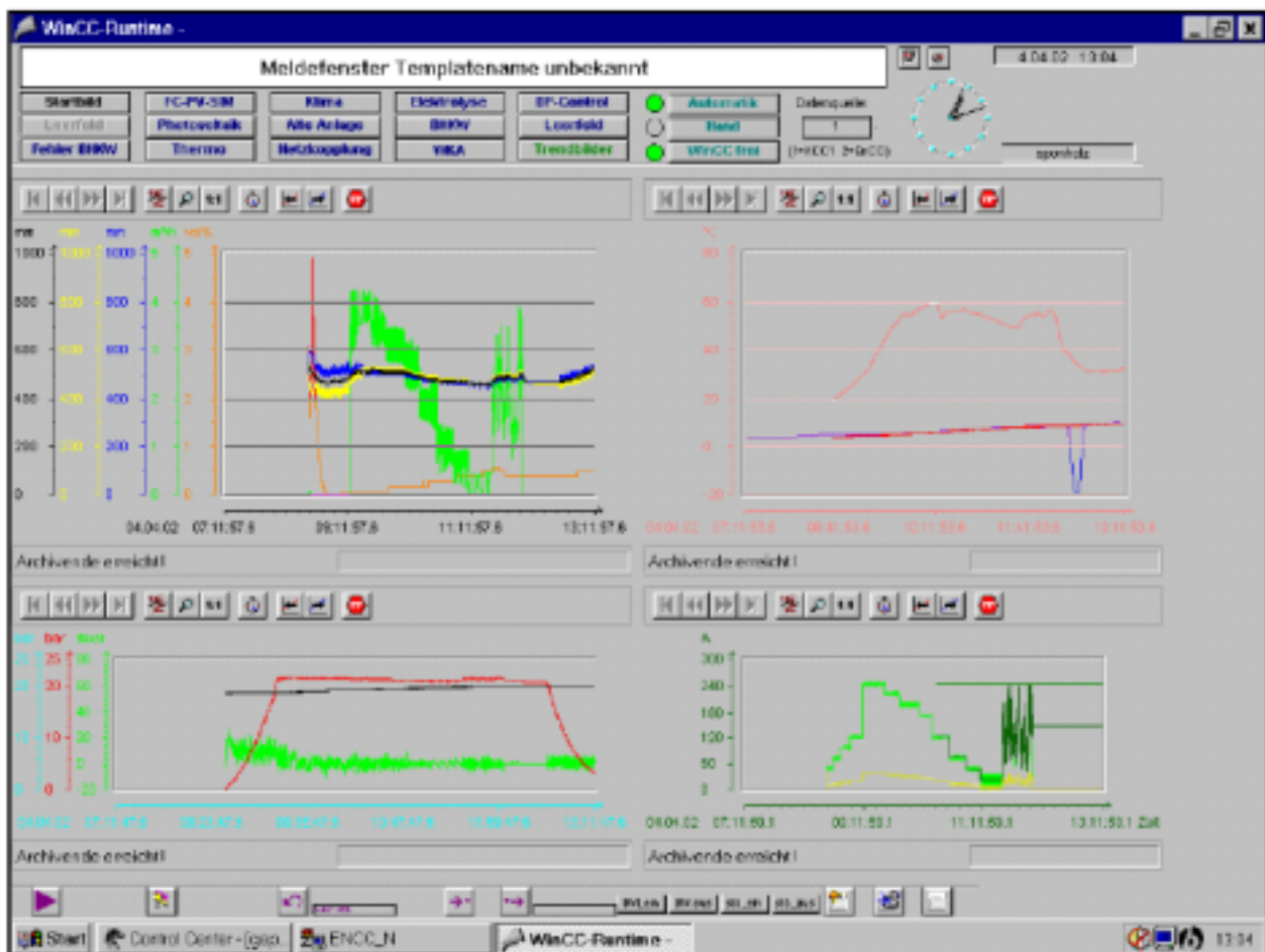
Figure 13. Data collection of the electrolyser
