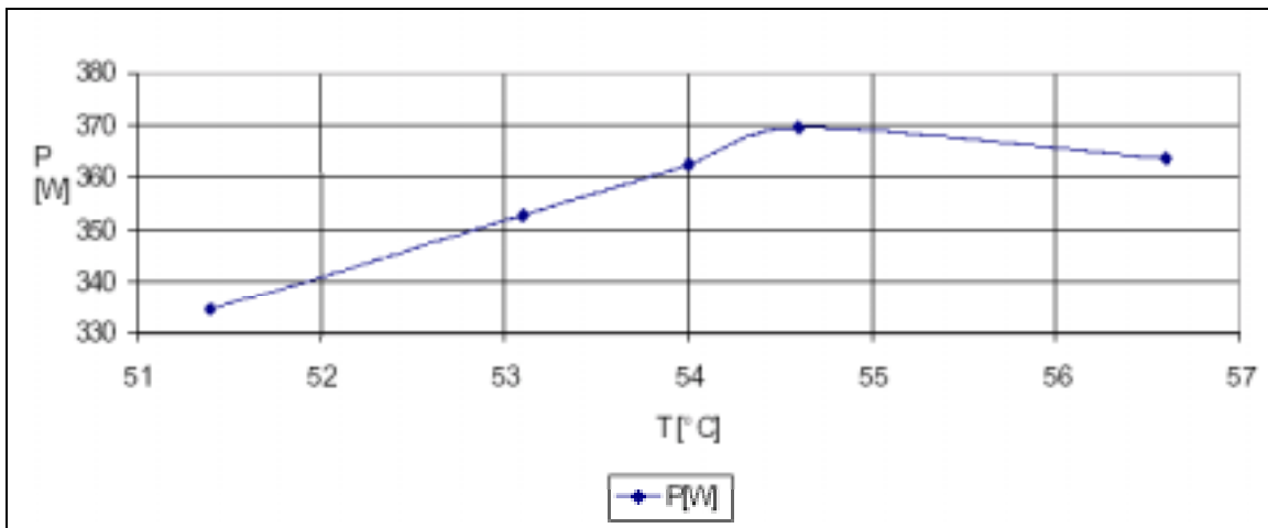
Figure 7: Temperature behavior of the PEM Fuel Cell
