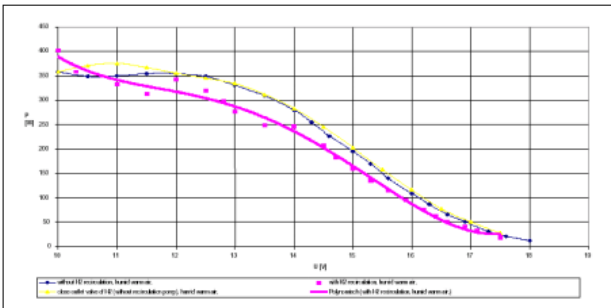
Figure 9: Power versus voltage
